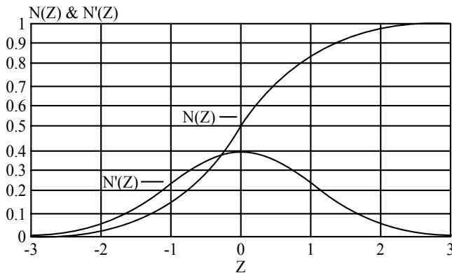
Figure 3-8 Equation (3.21) showing probability with Z = +2.
