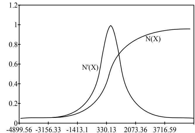
Figure 4-10 Adjustable distribution fit to the 232 trades.
