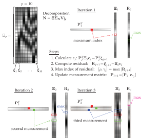
Figure 12.15 Demonstration of the first three iterations of the DEIM algorithm. For illustration only, the nonlinearity matrix N = \Xi \Sigma_N V_N^T is assumed to be composed of harmonic oscillator modes with the first ten modes comprising \Xi_p . The initial measurement location is chosen at the maximum of the first mode \xi_1 . Afterwards, there is a three step process for selecting subsequent measurement locations based upon the location of the maximum of the residual vector R_j . The first (red), second (green) and third (blue) measurement locations are shown along with the construction of the sampling matrix P
