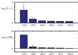
Figure 12.4 Logarithm of the least-square error, \log(E+1) (unity is added to avoid negative numbers), and the log of the condition number, \log(\kappa(\mathbf{M})) , as a function of percentage of random measurements. For 10% measurements, the error and condition number are largest as expected. However, the variance of the results, depicted by the red bars, is also quite large, suggesting that the performance for a small number of sensors is highly sensitive to their placement.
