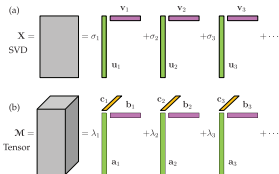
Figure 1.29 Comparison of the SVD and Tensor decomposition frameworks. Both methods produce an approximation to the original data matrix by sums of outer products. Specifically, the tensor decomposition generalizes the concept of the SVD to N -way arrays of data without having to flatten (vectorize) the data.
