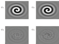
Figure 11.11 First four POD modes associated with the rotating spiral wave w(x, y) . The first two modes capture all the variance to numerical precision while the third and fourth mode are noisy due to numerical round-off. The domain considered is x \in [-20, 20] and y \in [-20, 20] .
