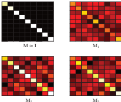
Figure 12.3 Demonstration of the deterioration of the orthogonality of the modal basis in the support space x[\bar{u}] as given by the matrix \mathbf{M} defined in (12.4). The top left shows that the identity matrix is produced for full measurements, or nearly so but with errors due to truncation of the domain over x \in [-4, 4] . The matrices \mathbf{M}_j , which longer look diagonal, correspond to the sparse sampling matrices \mathbf{P}_j in Fig. 12.1. Thus it is clear that the modes are not orthogonal in the support space of the measurements.
