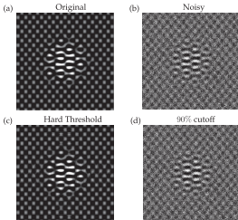
Figure 1.22 Underlying rank 2 matrix (a), matrix with noise (b), clean matrix after optimal hard threshold (4/\sqrt{3})\sqrt{\text{nr}} (c), and truncation based on 90% energy (d).
