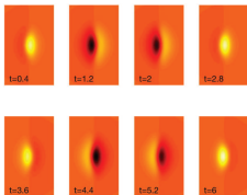
Figure 1.30 Example N -way array data set created from the function (1.45). The data matrix is \mathbf{A} \in \mathbb{R}^{121 \times 101 \times 315} . A CP tensor decomposition can be used to extract the two underlying structures that produced the data.
