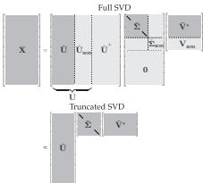
Figure 1.2 Schematic of truncated SVD. The subscript ‘ remain ’ denotes the remainder of \hat{U} , \hat{\Sigma} or \hat{V} after truncation.
