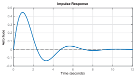
Figure 8.24 Impulse response of spring-mass-damper system.
