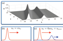
Figure 7.7 Inferring nonlinearity via observing solutions at multiple amplitudes (reproduced from Rudy et al. [460]). (a) An example 2-soliton solution to the KdV equation. (b) Applying our method to a single soliton solution determines that it solves the standard advection equation. (c) Looking at two completely separate solutions reveals nonlinearity.
