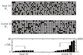
Figure 12.7 Depiction of the 10 best and 10 worst random 20% measurement vectors P_j considered in Figs. 12.5 and 12.6. The top panel shows that the best measurement vectors sample fairly uniformly across the domain x \in [-4, 4] with \Delta x = 0.1 . In contrast, the worst randomly generated measurements (middle panel) have large sampling gaps near the center of the domain, leading to a large condition number \kappa(M) . The bottom panel shows a bar chart of the best and worst values of the condition number. Note that with 20% sampling, there can be two orders of magnitude difference in the condition number, thus suggesting the importance of prescribing good measurement locations.
