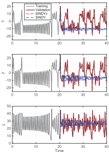
Figure 10.3 SINDY and SINDYc predictions for the controlled Lorenz system in (10.22). Training data consists of the Lorenz system with state feedback. For the training period the input is w(t) = 26 - x(t) + d(t) with a Gaussian disturbance d . Afterward the input w switches to a periodic signal w(t) = 50 \sin(10t) . Reproduced with permission from [100].
