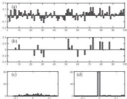
Figure 4.12 Solutions to an under-determined system with 20 constraints and 100 unknowns. Panels (a) and (b) show a bar plot of the values of the loadings of the vectors \mathbf{x} . In the former panel, the optimization is subject to minimizing the \ell_2 norm of the solution, while the latter panel is subject to minimizing the \ell_1 norm. Note that the \ell_1 penalization produces a sparse solution vector. A histogram of the loading values for (a) and (b) is shown in the panels (c) and (d) respectively.
