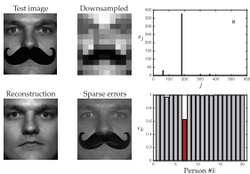
Figure 3.16 Sparse representation for classification demonstrated on example face from person 7th occluded by a fake mustache.
