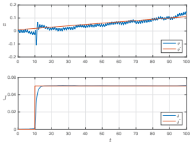
Figure 10.21 Extremum-seeking control response for a challenging test system with a right-half plane zero, inspired by [199].
