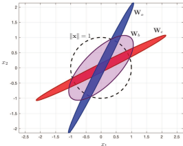
Figure 9.2 Illustration of balancing transformation on Gramians. The reachable set with unit control input is shown in red, given by W_c^{1/2}\mathbf{x} for \|\mathbf{x}\| = 1 . The corresponding observable set is shown in blue. Under the balancing transformation \mathbf{T} , the Gramians are equal, shown in purple.
