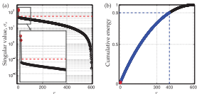
Figure 1.23 Singular values \sigma_r (a) and cumulative energy in first r modes (b). The optimal hard threshold \tau = (4/\sqrt{3})\sqrt{\bar{\sigma}}\sigma is shown as a red dashed line (- -), and the 90% cutoff is shown as a blue dashed line (- -). For this case, n = 600 and \sigma = 1 so that the optimal cutoff is approximately r = 56.6 .
