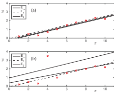
Figure 4.2 Line fits for the three different error metrics E_{\infty} , E_1 and E_2 . In (a), the data has not outliers and the three linear models, although different, produce approximately the same model. With outliers, (b) shows that the predictions are significantly different.
